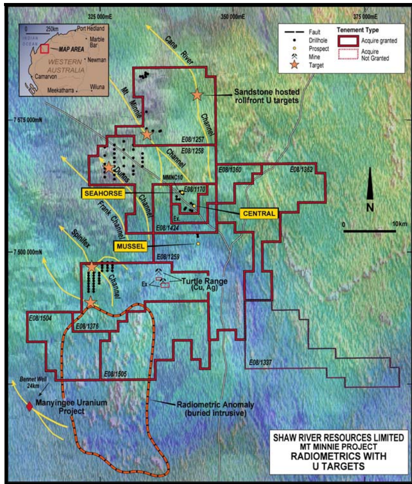
Mt Minnie Tenements, showing palaeochannels.
